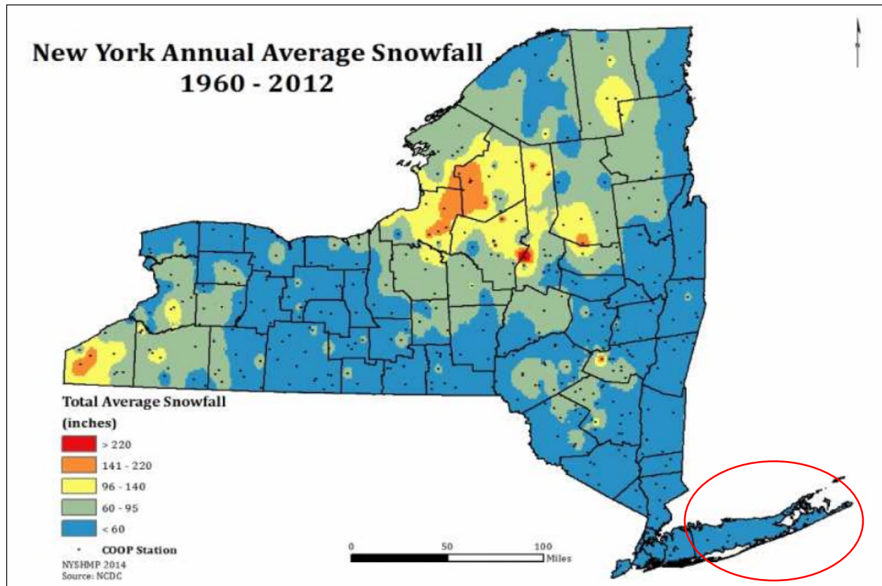
Figure 5.4.14-1. Annual Average Snowfall for New York State
